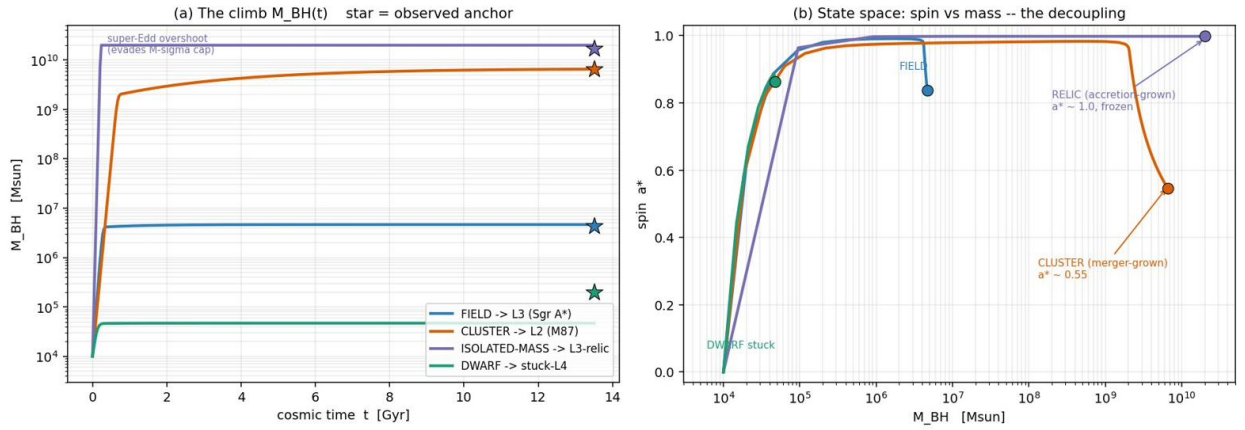
Figure 1: (a) The climb M_\bullet(t) : one set of equations, four environments, four fates; stars are observed anchors (Sgr A*, M87, NGC 1277, dwarf IMBHs; the NGC 1277 star is drawn at the superseded 2012 anchor — the corrected Walsh 2016 mass is 4.9 \times 10^9 M_\odot , see table footnote). (b) State space a_* vs M_\bullet : at fixed \sigma = 300 the cluster (merger-grown) lands at a_* \approx 0.55 while the relic (accretion-grown) freezes at a_* \approx 1.0 .
