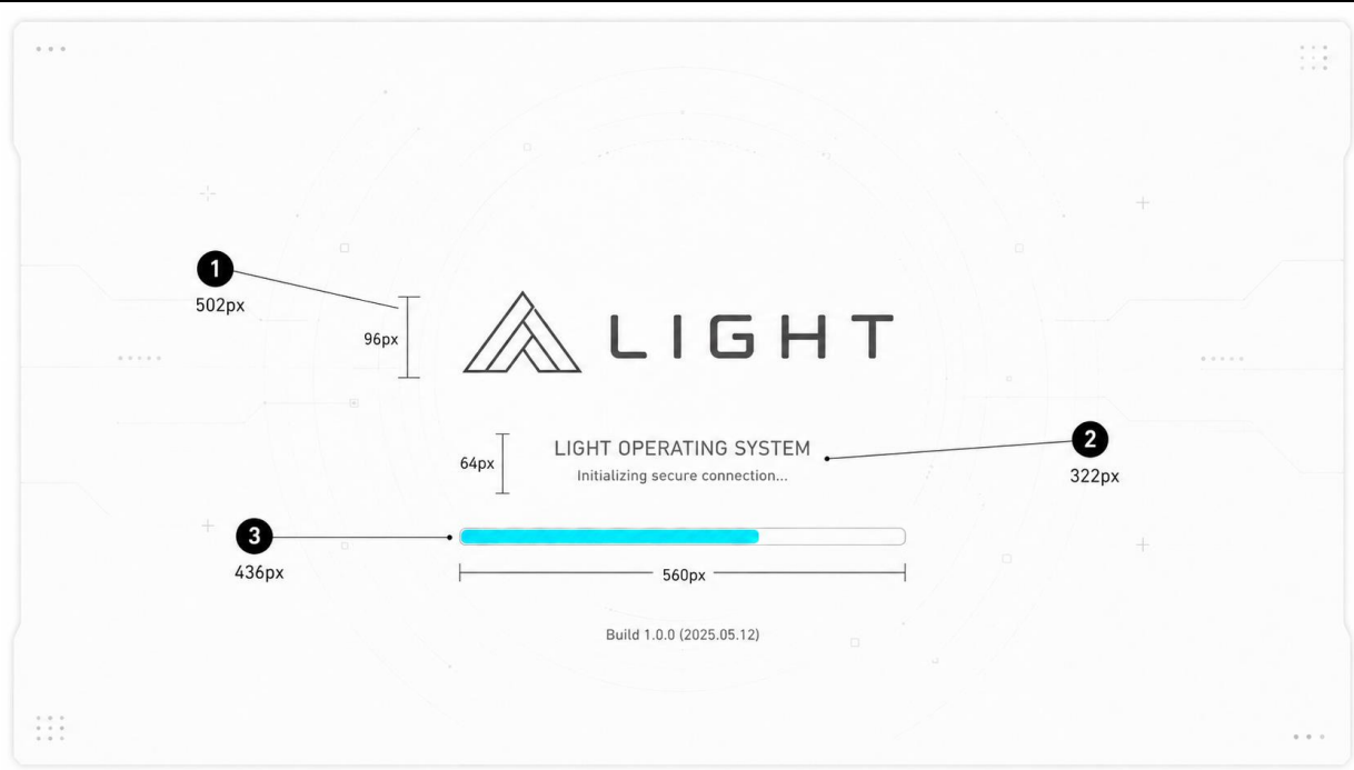
S001 Splash
