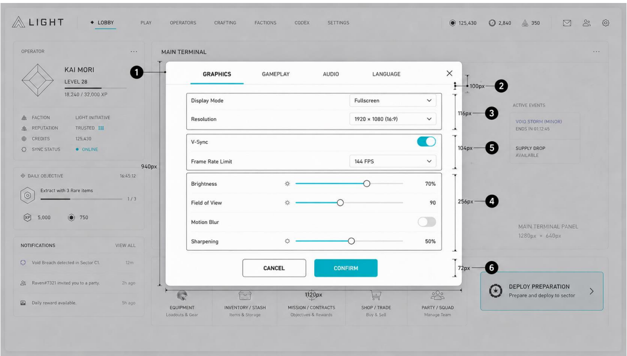
S004 Settings
