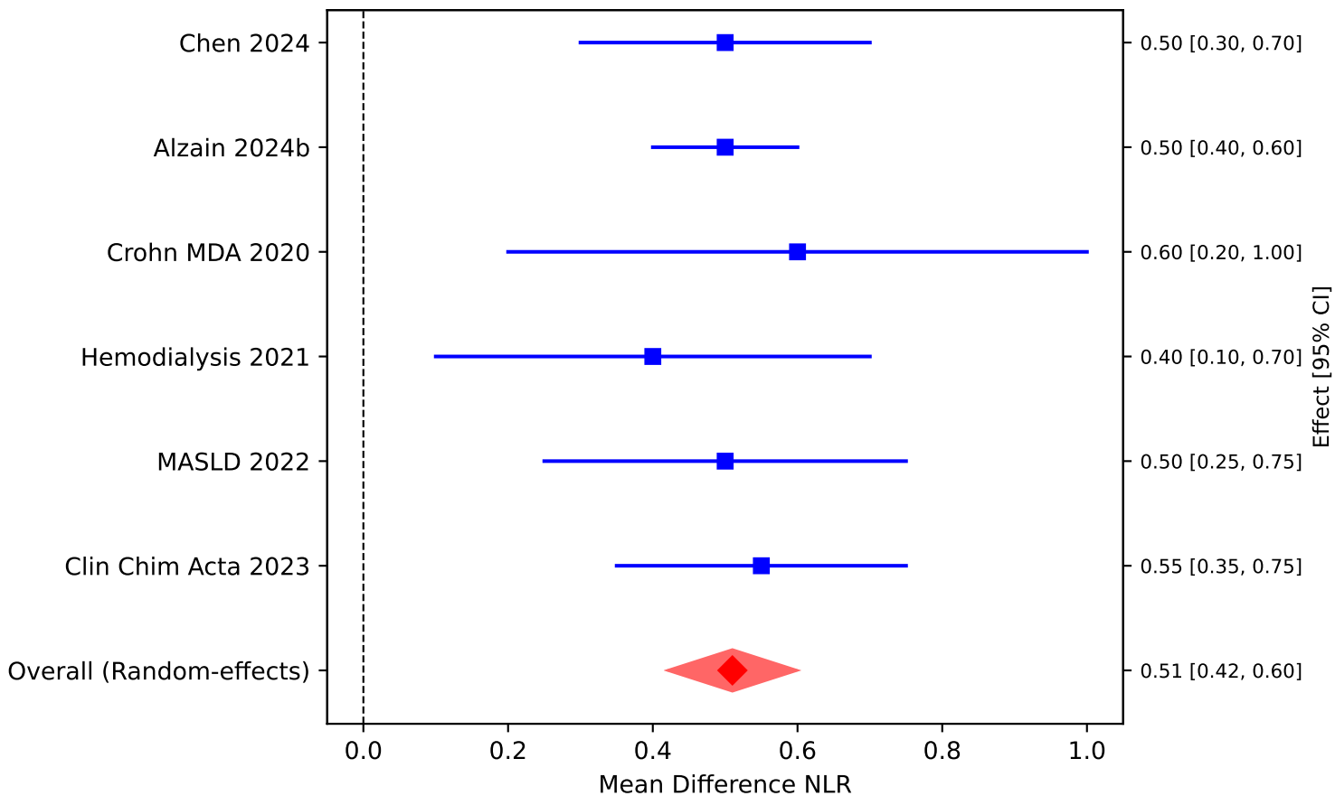
Fig S3 Forest plot: NLR SHS vs Healthy (Random-effects I 2 =15%, p<0.001)
