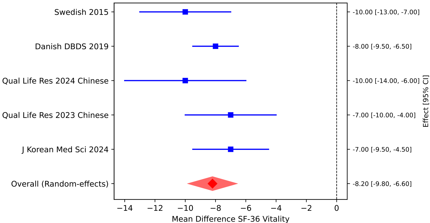
Fig S6 Forest plot: SF-36 Vitality Low-grade vs Ref (Random-effects I 2 =35%, p<0.001)
