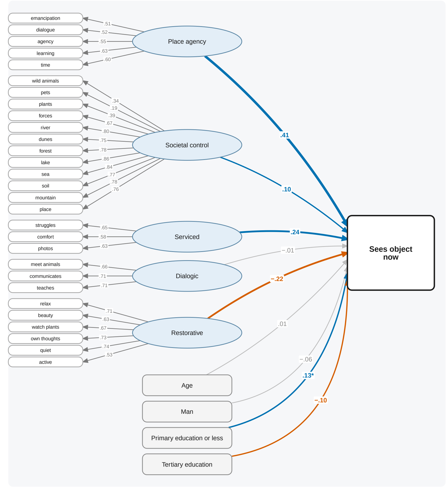
The role people SEE (R² = 0.22)
