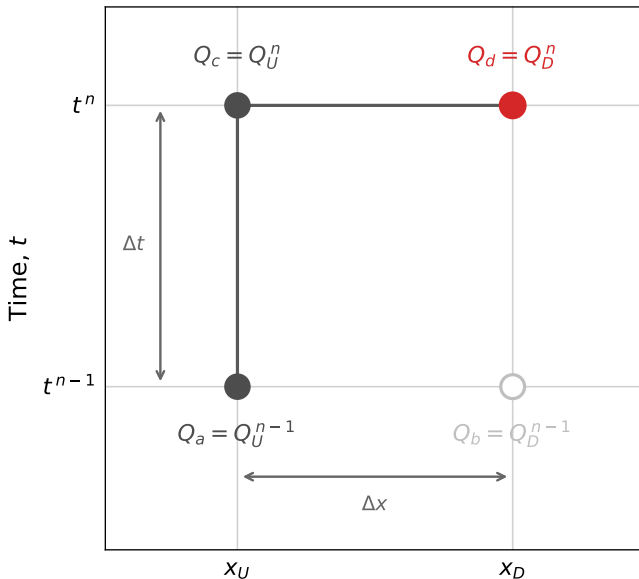
B C_r > 1 : upstream-only storage stencil
