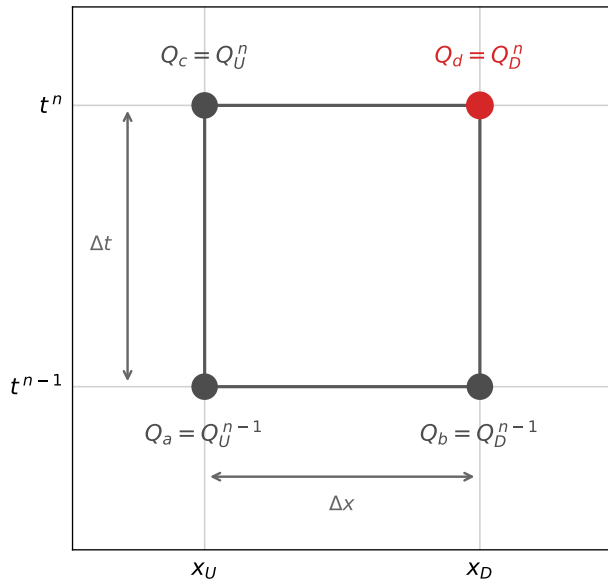
A C_r \leq 1 : four-point weighted stencil
