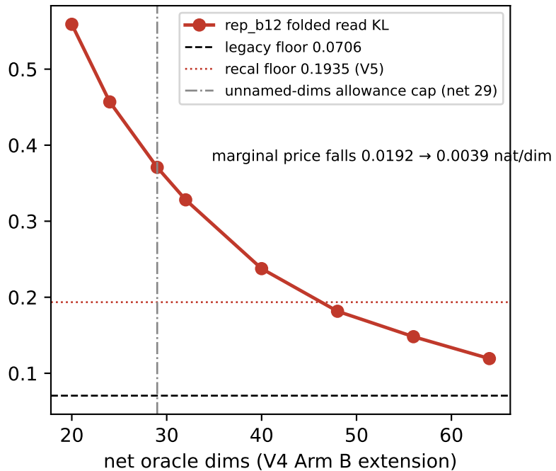
V4: rep_b12 plateaus above the legacy floor; closes only under the honest recal meter (V5)
