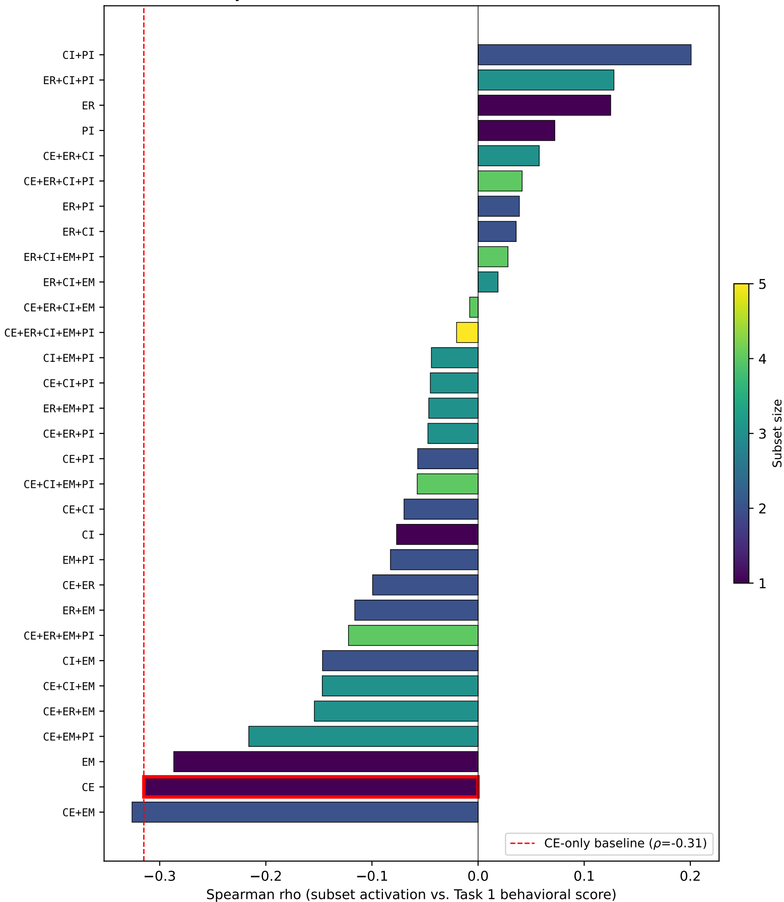
MSV dimension-subset routing quality (23-model Kaggle cohort) CE-only baseline outlined in red. Bar color = subset size.
