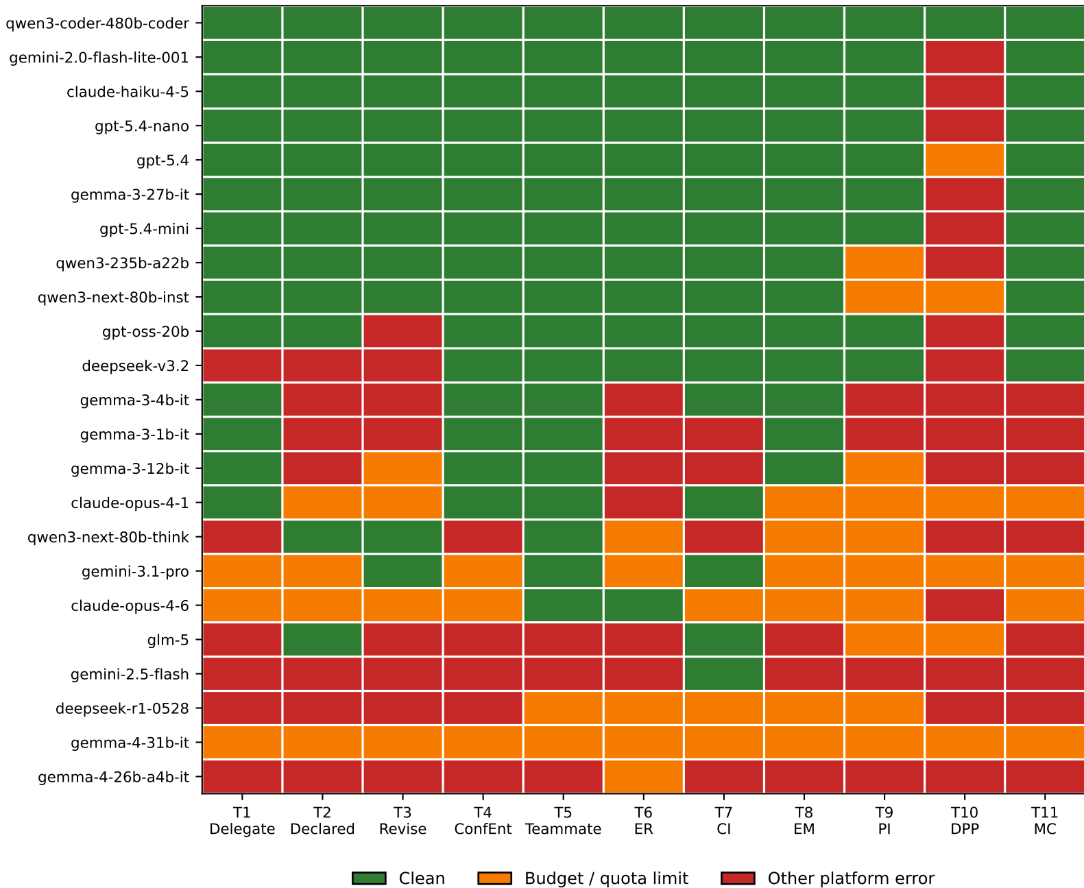
Kaggle benchmark completion picture: 23 models x 11 tasks = 253 runs 133 clean (53%), 50 budget/quota (20%), 70 other errors (28%)
