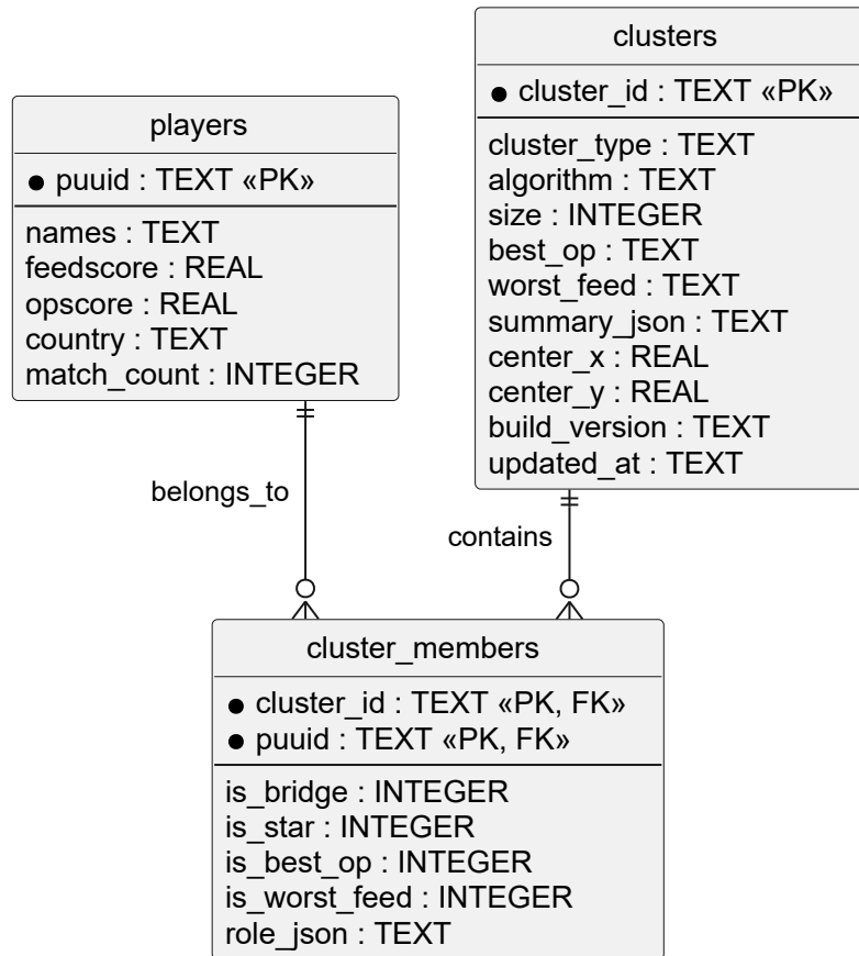
4.3. ábra: Relational model for cluster and player persistence ( players , clusters , cluster_members )
