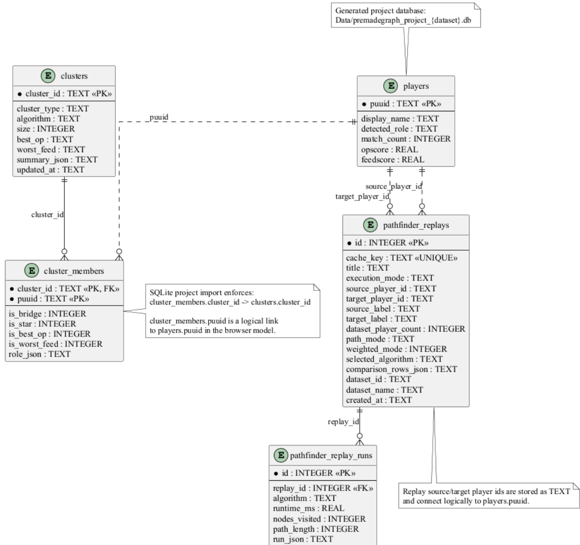
4.2. ábra: Entity-relationship diagram of the main SQLite database
