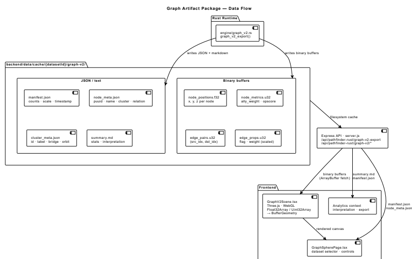
7.2. ábra: Data flow of the graph artifact package: the Rust exporter writes binary and JSON layers, Express serves them, and the frontend consumes them in a WebGL renderer
