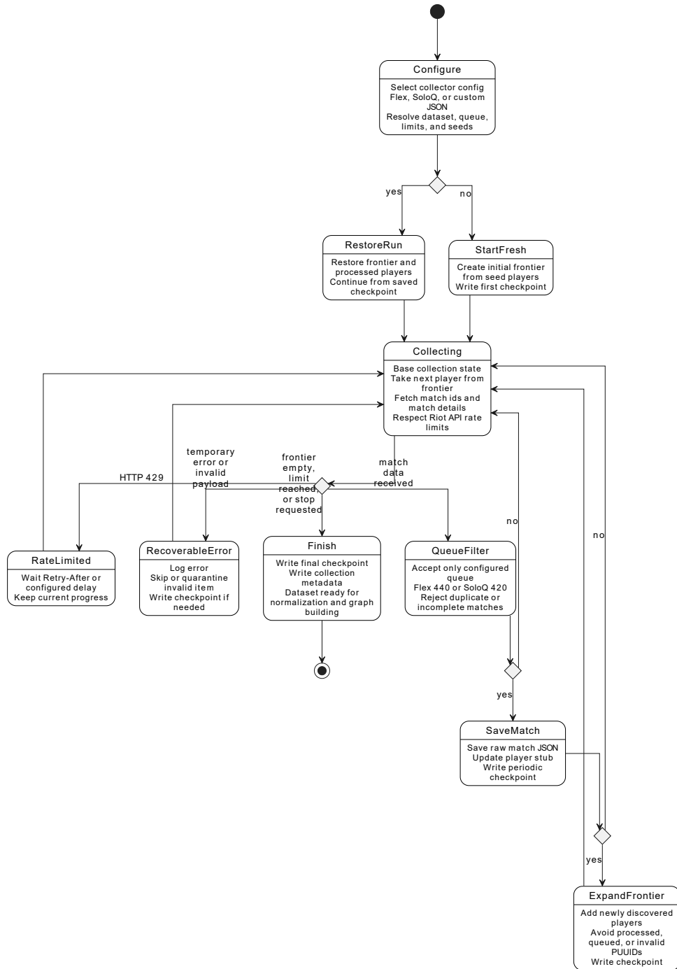
Match Collector State Flow -- Rate Limits, Checkpoints, Seed Expansion, and Queue Filtering
