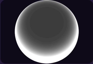
assets/kenney/2D assets/Planets/Parts/light7.png
