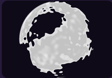
assets/kenney/2D assets/Planets/Parts/noise27.png
