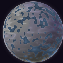
assets/kenney/2D assets/Planets/Planets/planet04.png
