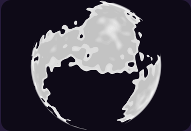
assets/kenney/2D assets/Planets/Parts/noise26.png
