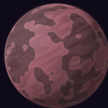
assets/kenney/2D assets/Planets/Planets/planet06.png
