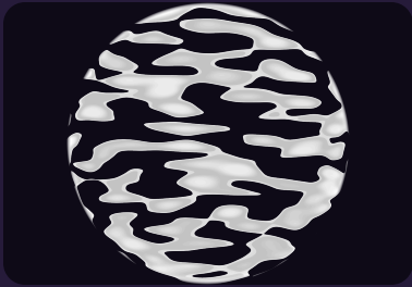
assets/kenney/2D assets/Planets/Parts/noise12.png
