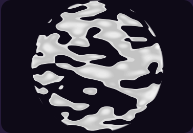
assets/kenney/2D assets/Planets/Parts/noise09.png
