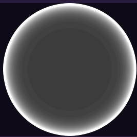
assets/kenney/2D assets/Planets/Parts/light4.png
