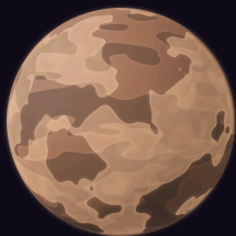
assets/kenney/2D assets/Planets/Planets/planet05.png
