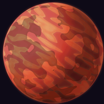
assets/kenney/2D assets/Planets/Planets/planet08.png
