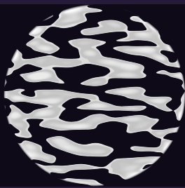
assets/kenney/2D assets/Planets/Parts/noise14.png
