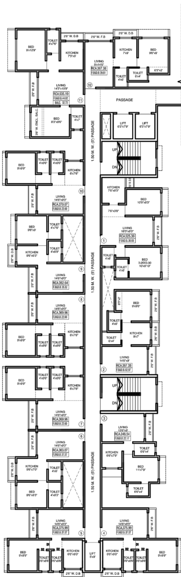
3RD, 5TH, 7TH, 9TH, 11TH, 15TH, 17TH, 19TH & 21TH FLOOR PLAN
