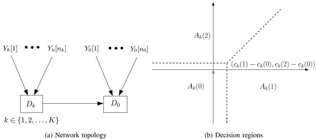
Fig. 2. A tandem network and its decision regions.
