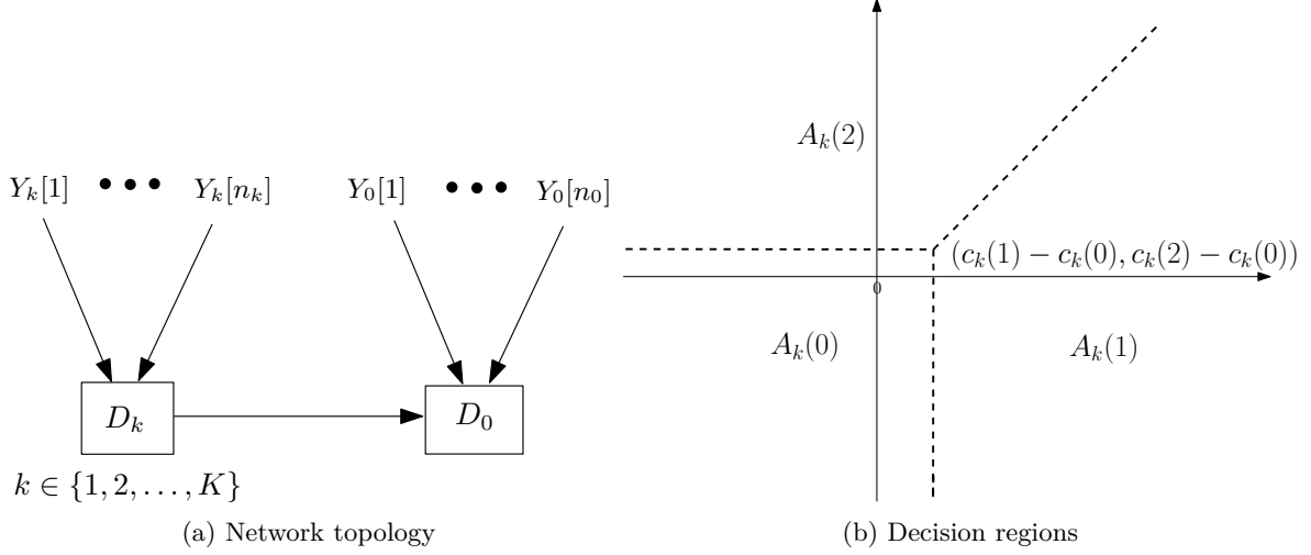
Fig. 2. A tandem network and its decision regions.
