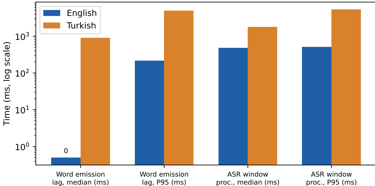
Layer 1 latency: English vs. Turkish (Table 6)
