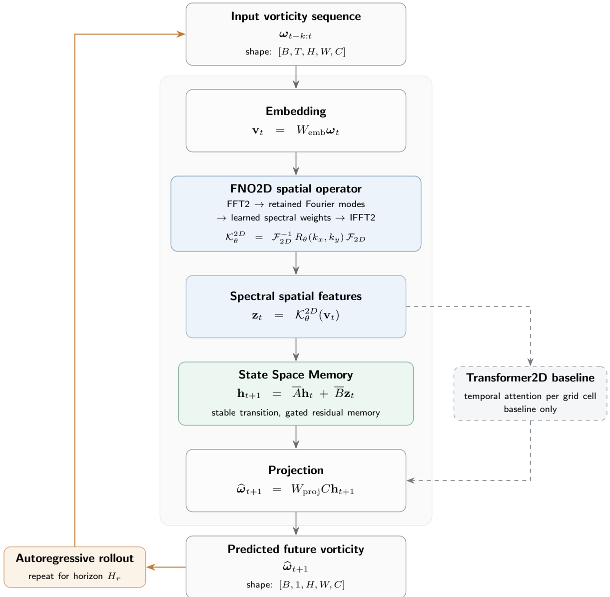
SM-FNO2D separates 2D PDE forecasting into spectral spatial mixing with FNO2D and attention-free temporal memory with an SSM. The figure is an architectural overview, not a performance claim.
