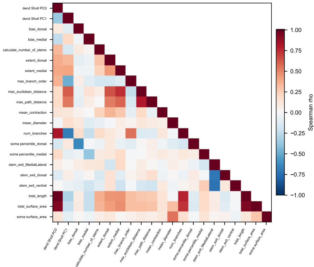
Macaque MSN primary21 Spearman correlation
