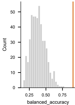
Within-donor permutation
