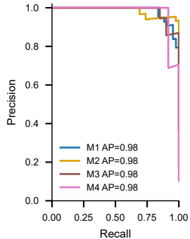
One-vs-rest PR
