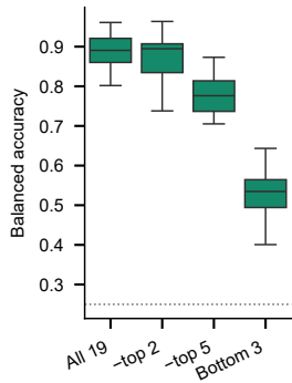
Nested feature ablation
