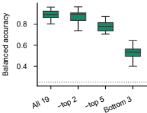
Nested feature ablation
