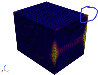
Shear xz (gamma_xz=1)
