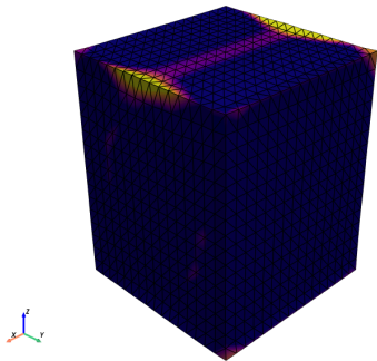
Shear xy (gamma_xy=1)
