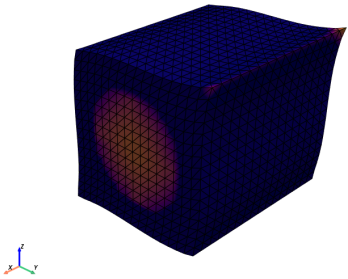
Shear yz (gamma_yz=1)
