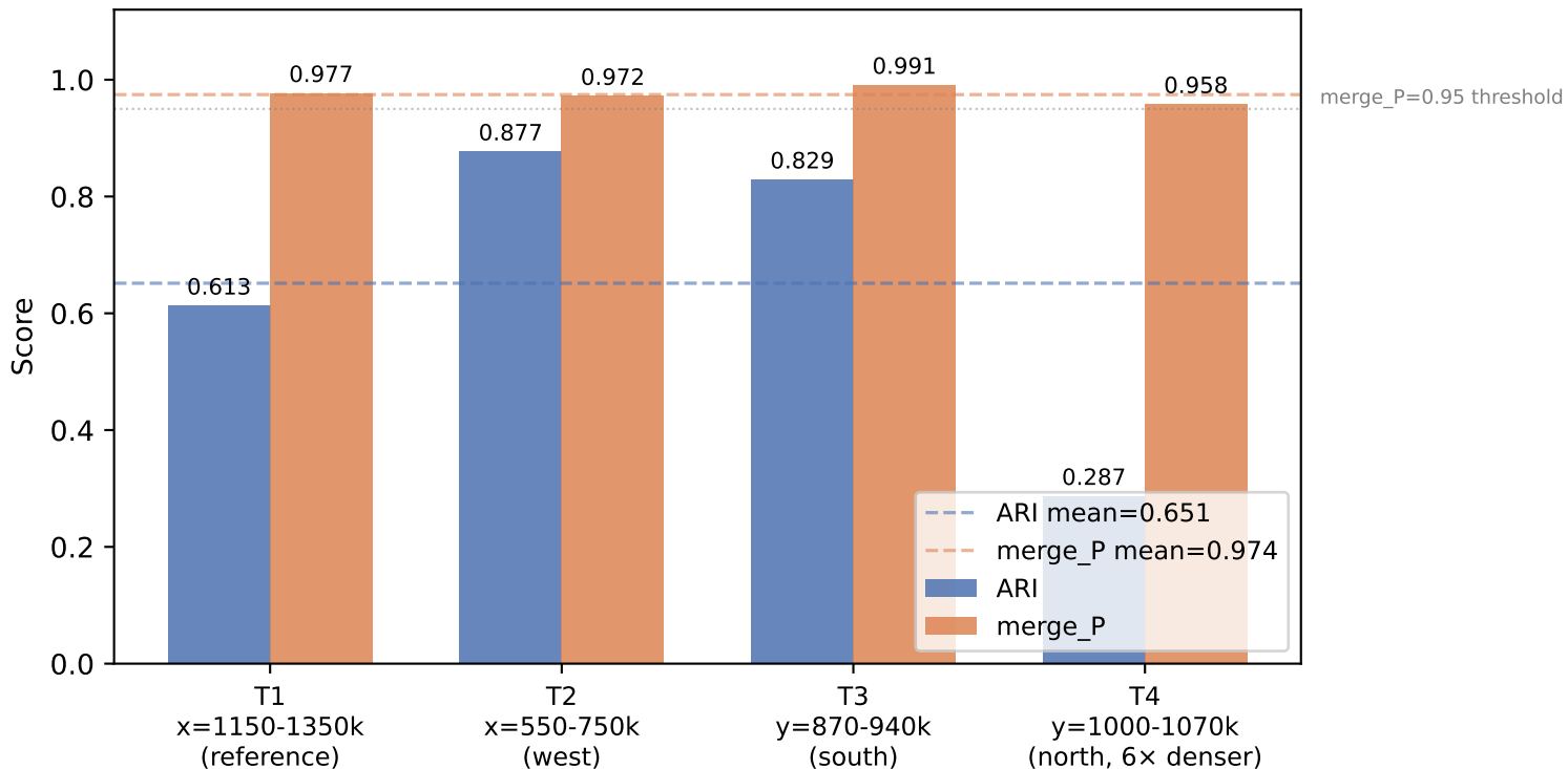
Spatial variance: ARI and merge_P across 4 in-column test bboxes (same A/B/C-trained model, 50 \mu m seam buffer, b = -2.0 )
