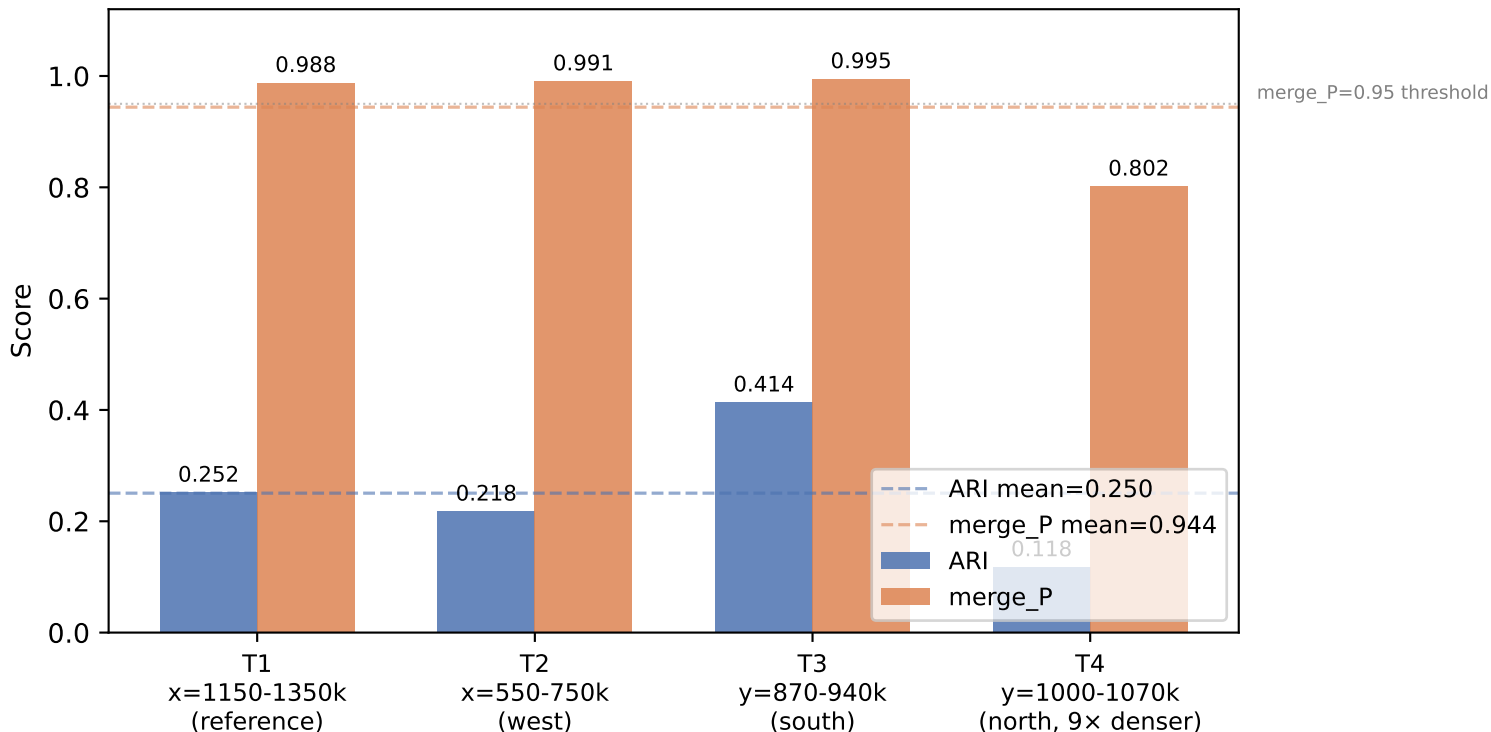
Spatial variance: ARI and merge_P across 4 in-column test bboxes (dual-side trained model, A/B/C pre+post, 50 \mu m seam buffer, b = -2.0 )
