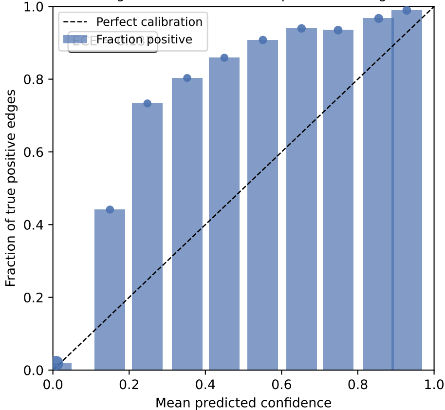
Reliability diagram (T=1.095, ECE=0.137) EdgePartitionGNN after temperature scaling
