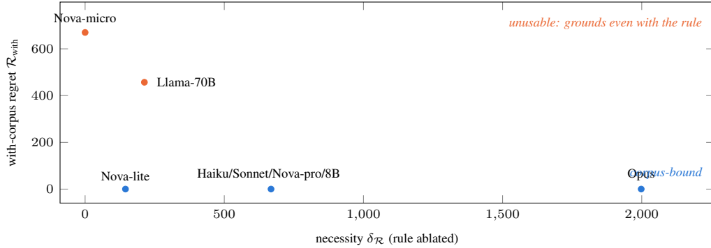
Figure 3: The necessity–usability plane for the eight models of Table 4 on the corpus-only hazard. Horizontal : necessity \delta_{\mathcal{R}} (how much ablating the rule raises regret; a coarse ordinal set by the fixed geometry—the four blue points at \delta_{\mathcal{R}} \approx 668 are four models that emit the same avoidance angle). Vertical : with-corpus regret— \approx 0 (blue, on the axis) means the model clears once given the rule ( usable ); a large value (orange) means it grounds even with the rule present ( unusable ). Reliance and usability are distinct axes: Claude Opus reads the corpus-only fact and clears, while Nova-micro and Llama-70B ground regardless.
