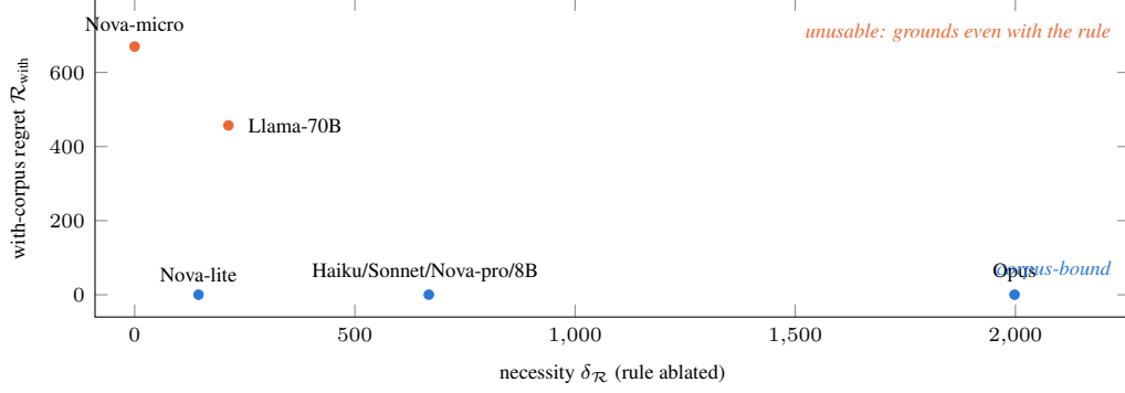
Figure 3: The necessity–usability plane for the eight models of Table 5 on the corpus-only hazard. Horizontal : necessity \delta_{\mathcal{R}} (how much ablating the rule raises regret; a coarse ordinal set by the fixed geometry—the four blue points at \delta_{\mathcal{R}} \approx 668 are four models that emit the same avoidance angle). Vertical : with-corpus regret— \approx 0 (blue, on the axis) means the model clears once given the rule ( usable ); a large value (orange) means it grounds even with the rule present ( unusable ). Reliance and usability are distinct axes: Claude Opus reads the corpus-only fact and clears, while Nova-micro and Llama-70B ground regardless.
