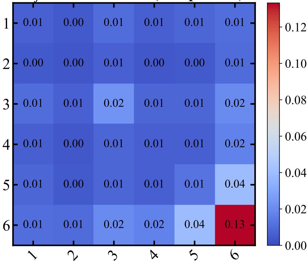
a_{ij} — HfNbTaTi (sample 7/9)
