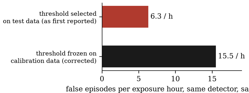
Figure 2: The audit’s effect. The same detector on the same data, with only the provenance of the operating threshold changed: selecting the threshold on test outcomes understated the false-alarm cost by a factor of approximately 2.5.
