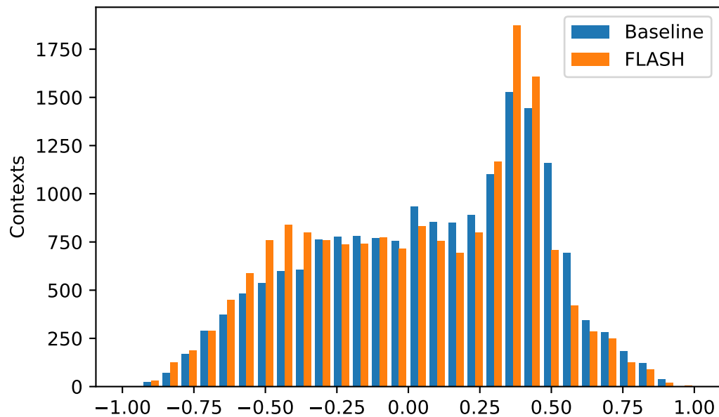
kendall: matched context correlations
