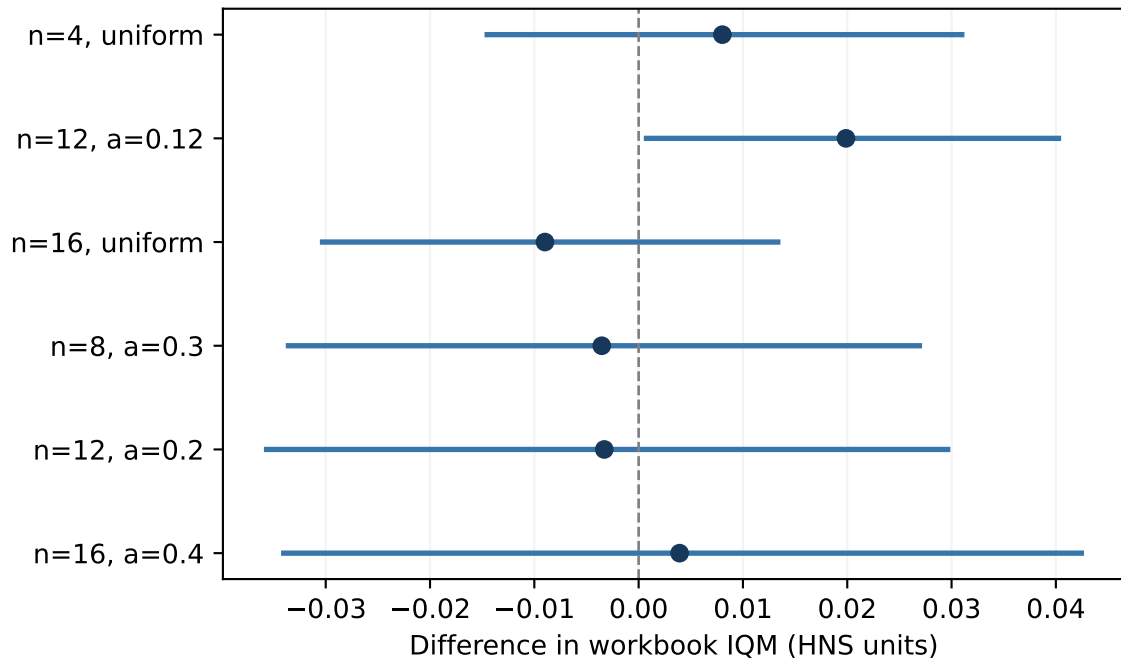
vs STORM
