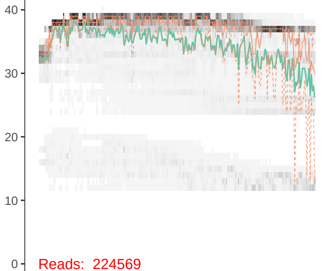
SRR12672863_1.fastq.gz
