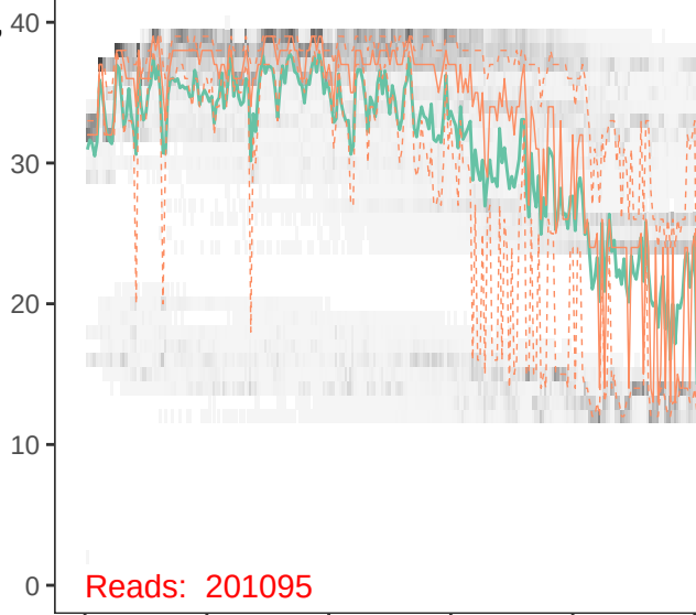
SRR12672863_2.fastq.gz
