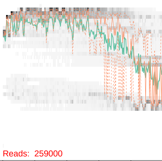
SRR12672864_2.fastq.gz
