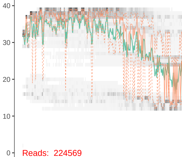
SRR12672863_2.fastq.gz
