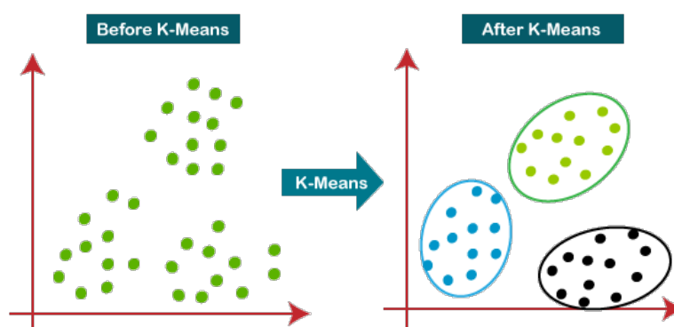
Figure 18.4: K-means alternates between assigning observations to centroids and moving centroids to cluster means.
