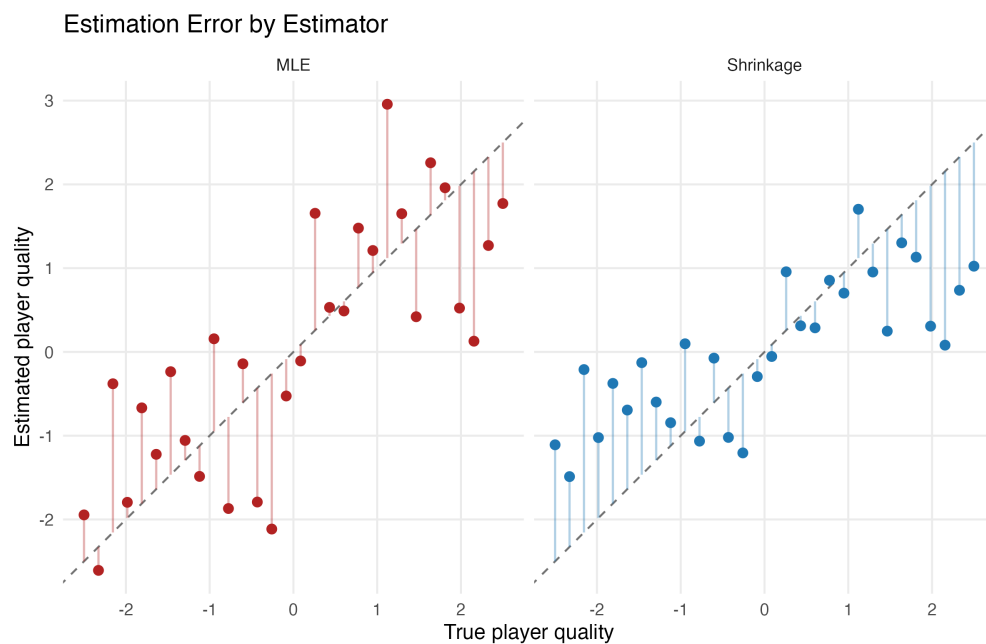
Figure 13.1: True and estimated player quality under the MLE and shrinkage estimator.
