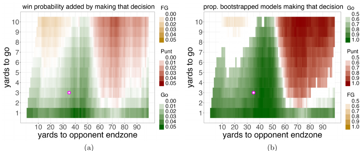
Figure 20.2: Decision boundary charts from Brill's fourth down decision model. Panel (a) shows the estimated win probability added by the recommended decision; panel (b) shows the proportion of bootstrap refits in which that decision remains optimal.
