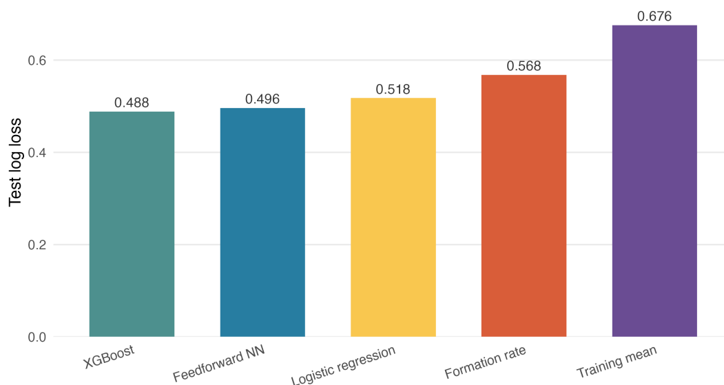
Figure 17.4: Test log loss for snap-frame dropback prediction.
