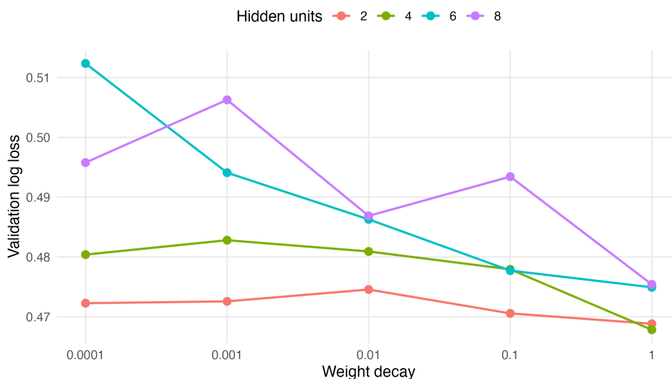
Figure 17.3: Validation log loss for one-hidden-layer feedforward networks with 2, 4, 6, or 8 hidden units and weight-decay penalties from 0.0001 to 1.
