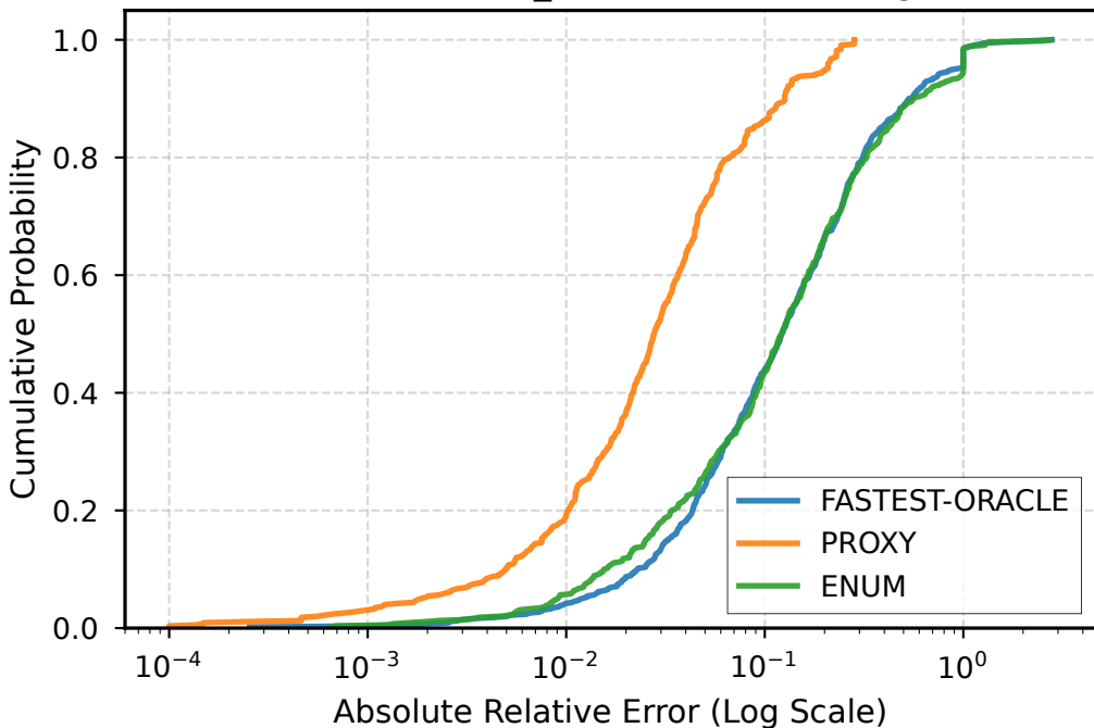
CDF of ARE (dataset_test - COUNT) - Budget 10%
