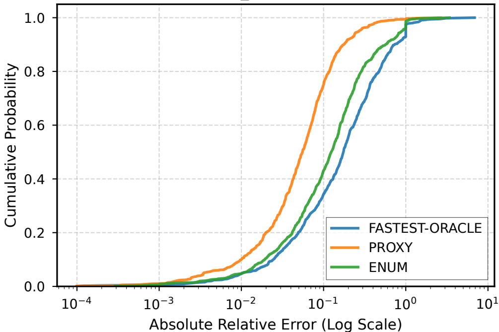
CDF of ARE (amazon_extend - SUM) - Budget 10%
