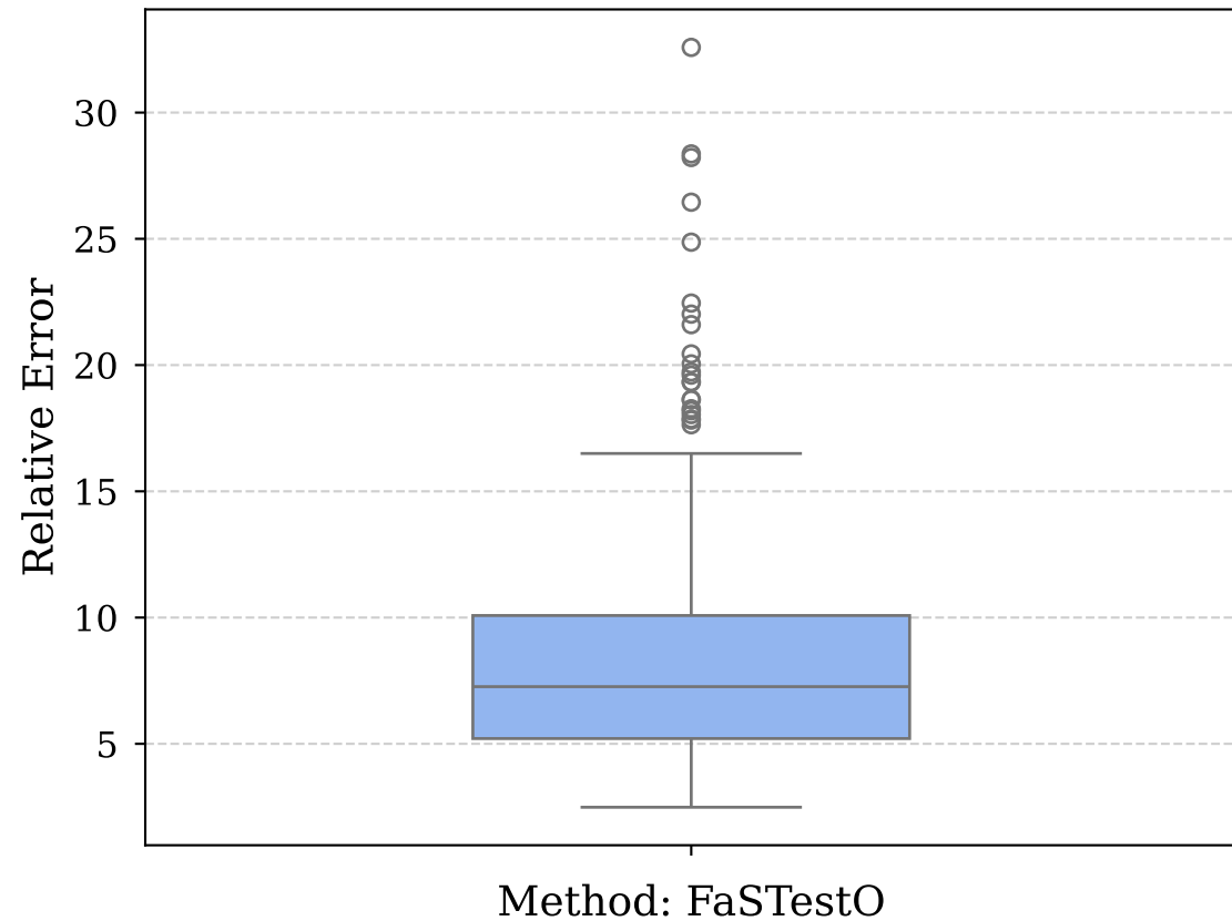
Error Distribution
