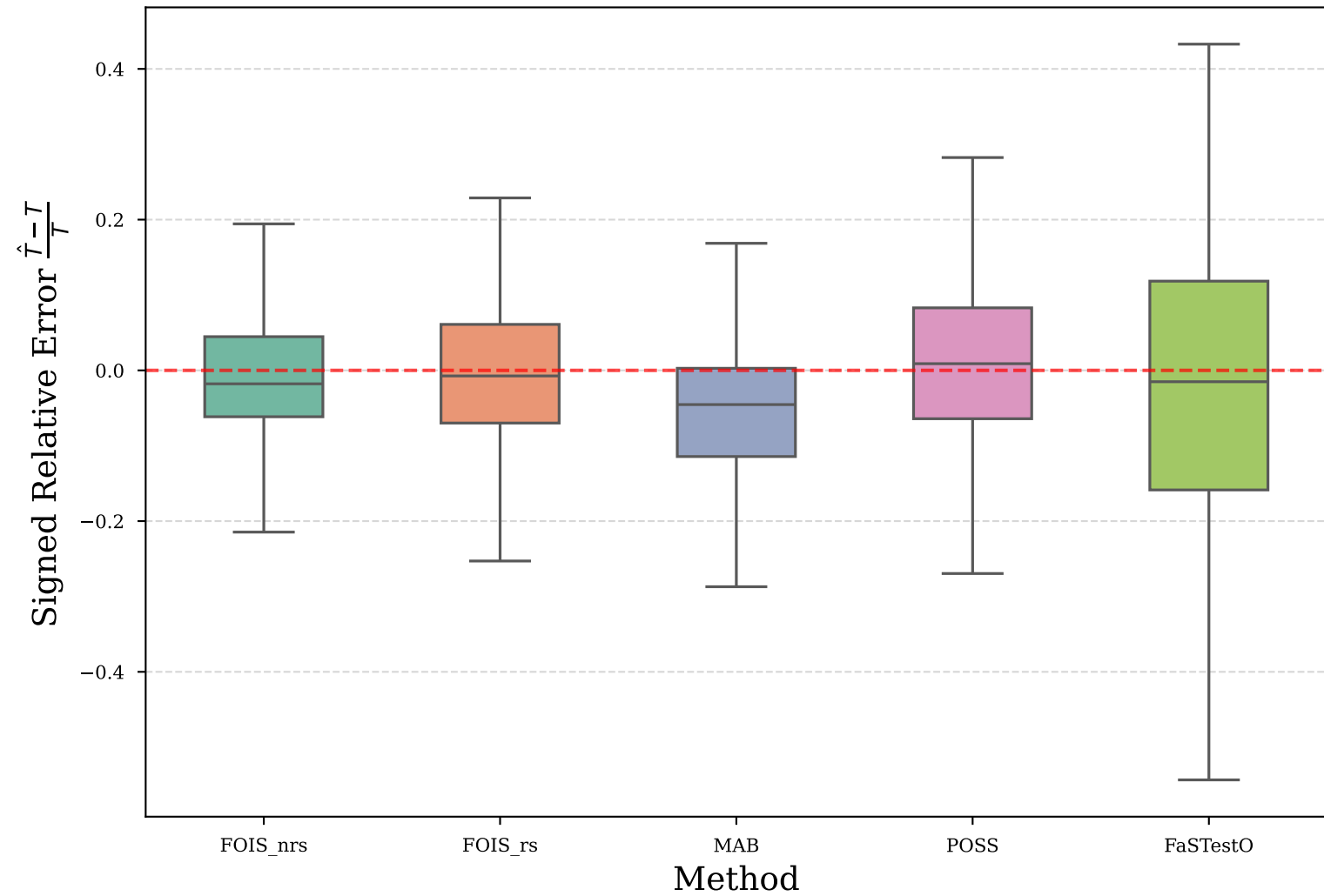
Bias Analysis (Signed Relative Error)
