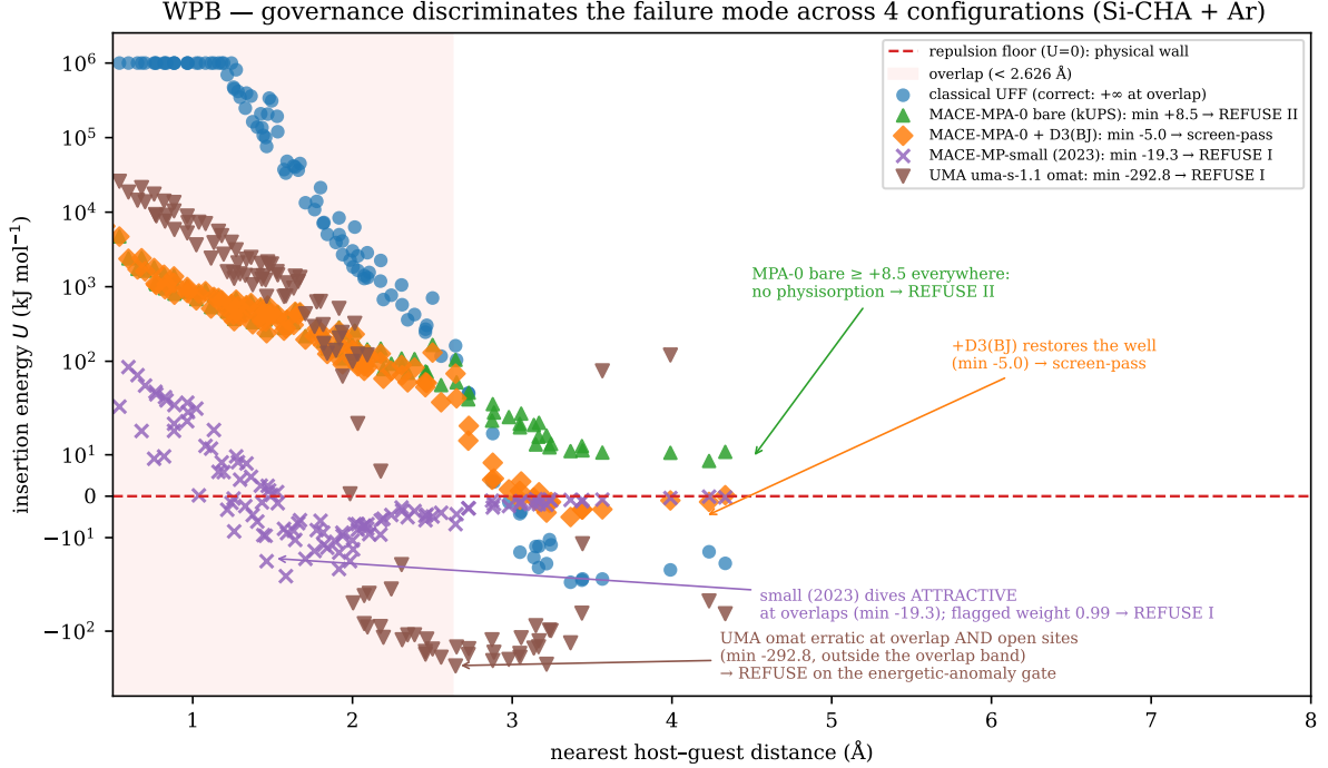
Figure 7: Out-of-distribution governance discriminates the failure mode across four configurations (Si-CHA + Ar). MACE-MP-small over-binds inside overlaps (refused); MACE-MPA-0 bare is repulsive everywhere, finding no physisorption well (refused); the same weights with D3(BJ) recover a physical well (screen-pass); the UMA materials head is erratic both inside and outside the overlap region and is refused on the energetic-anomaly gate. The shaded band is the corrected 2.626 Å hard-overlap threshold. Every label renders from a committed JSON.
