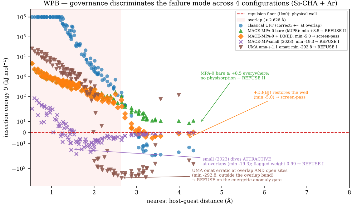
Figure 1: WPB — governance discriminates the failure mode across four configurations (Si-CHA + Ar).
