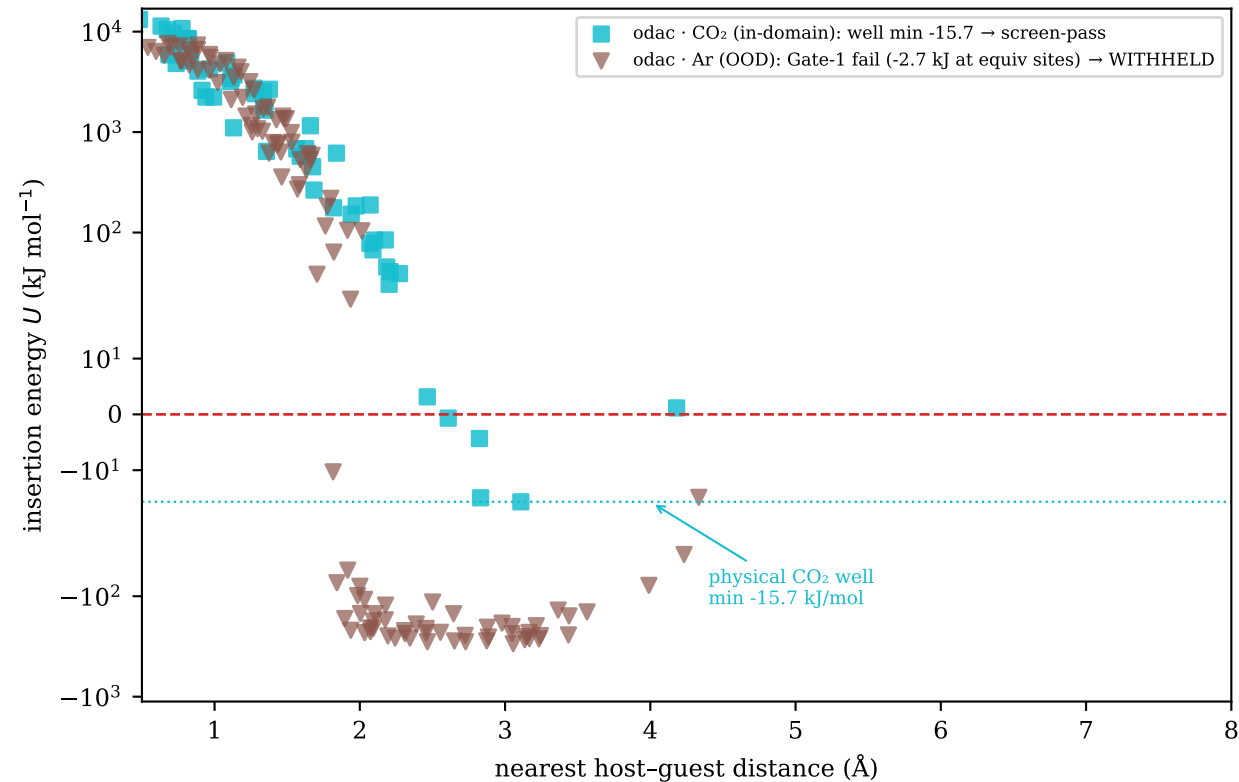
(A) odac head: in-domain CO 2 vs out-of-domain Ar (N=60)
