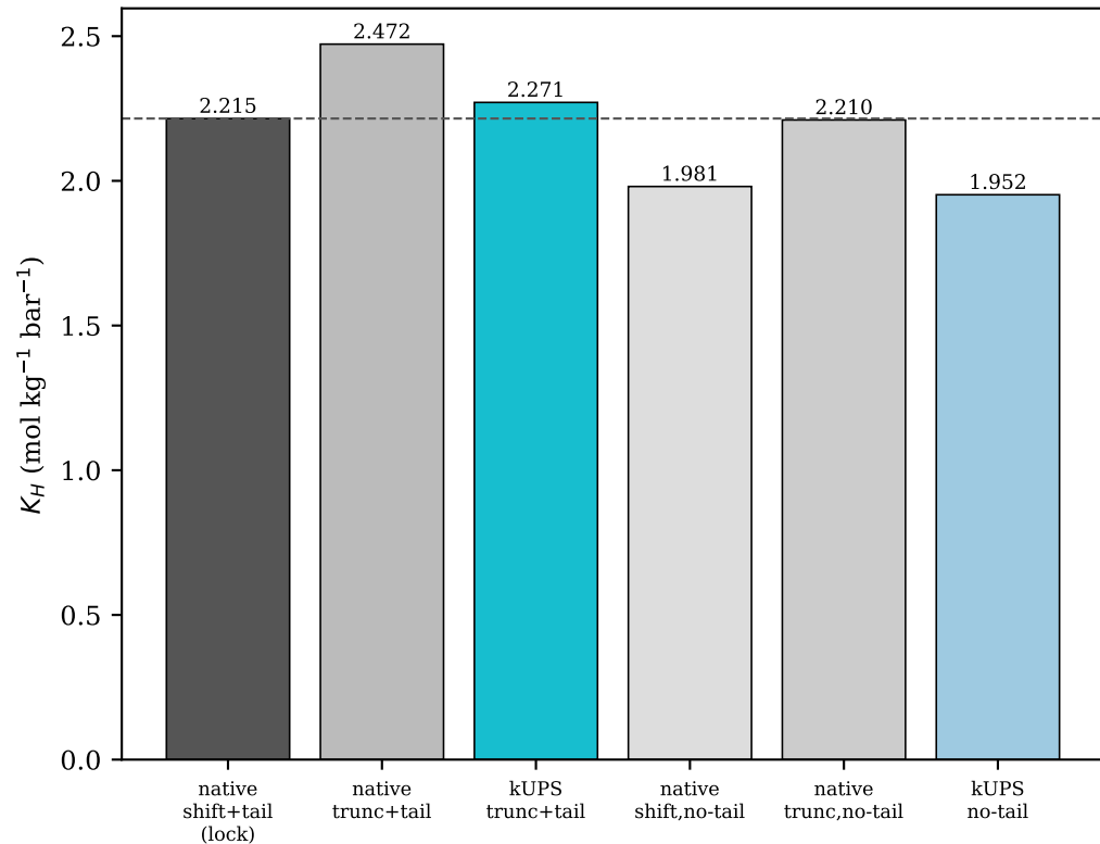
(B) 4c CHA+CO 2 (Ewald): shift +11.6%, tail +11.9%; kUPS matched-convention residual -8.1% (q st -invariant)
