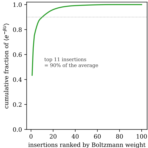
B. A few OOD insertions dominate K_H
