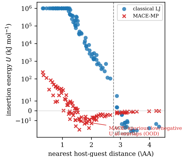
A. Classical repels overlaps; MACE does not
