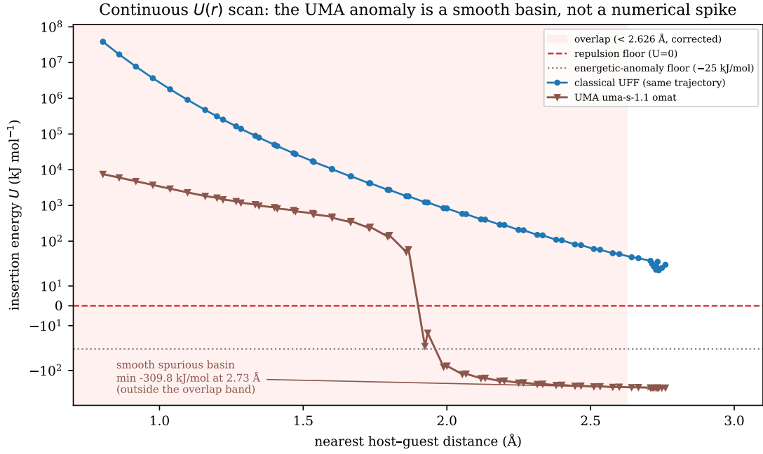
Figure 1: Continuous U(r) scan for UMA uma-s-1.1 (omat) on Si-CHA + Ar, along the line from the nearest framework oxygen through the deepest committed insertion. The classical comparator (blue) is monotonically repulsive over the whole range; the machine-learned potential (brown) crosses zero near 1.9 Å and falls into a smooth spurious basin reaching -309.8 kJ/mol at 2.73 Å, outside the corrected overlap band. Shading marks the corrected hard-overlap threshold; the dotted line is the energetic-anomaly floor. Every UMA value is read from the committed scan JSON.
