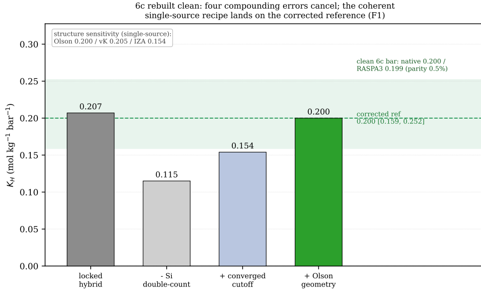
Figure 3: Finding F1 — branch 6c rebuilt clean. The originally-locked hybrid recipe (0.207) agrees with the reference only as a fortuitous cancellation of four compounding errors; removing the silicon double-count, converging the cutoff, and adopting Talu’s calibration (Olson) geometry lands the coherent single-source recipe on the corrected reference K_H = 0.200 , cross-engine (native 0.200, RASPA3 0.199; parity 0.5%). Values read from cancellation_6c.json .
