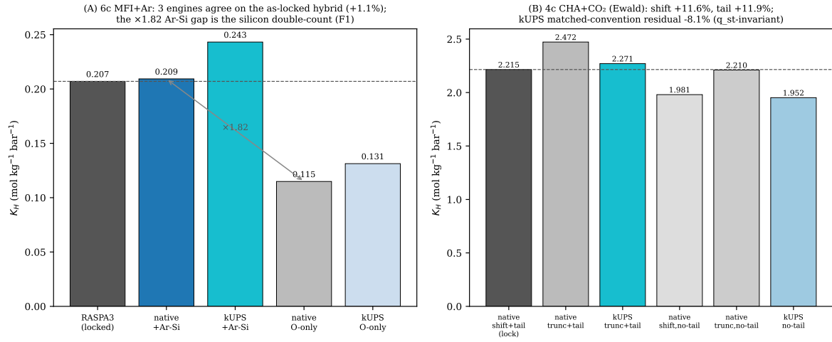
Figure 4: Cross-engine Widom parity: 6c three-way (native+Ar-Si reproduces RASPA3; the 1.8 \times gap to O-only is the silicon double-count of Finding F1) and the 4c CHA+CO 2 convention matrix (shift / tail toggles).
