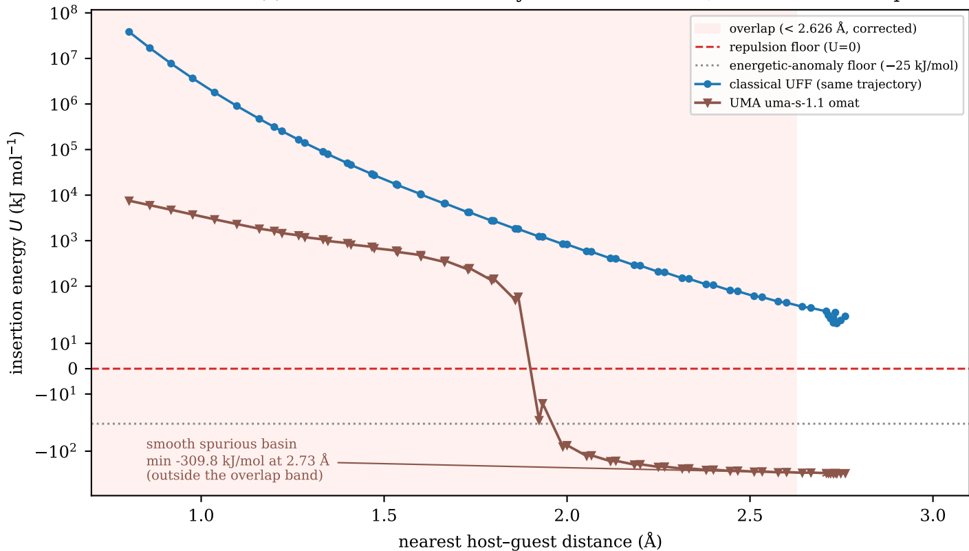
Continuous U(r) scan: the UMA anomaly is a smooth basin, not a numerical spike
