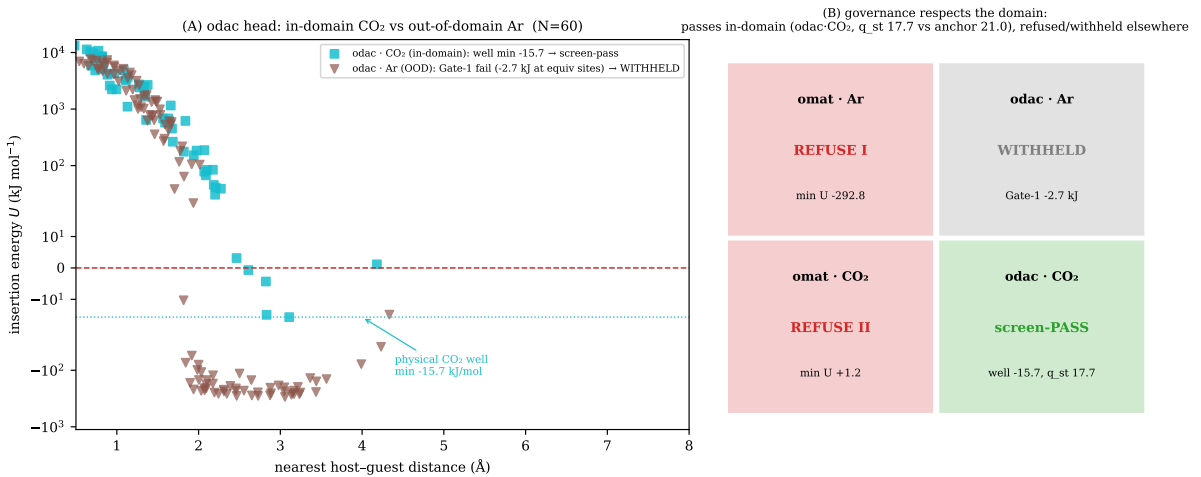
Figure 8: Governance respects the model’s domain. Left: the UMA direct-air-capture head screen-passes on \text{CO}_2 (adsorbate-in-domain; a physical well) and is withheld out-of-domain on Ar (internally inconsistent). Right: the full task-by-system verdict matrix; the model passes where its adsorbate domain holds and is refused or withheld elsewhere.
