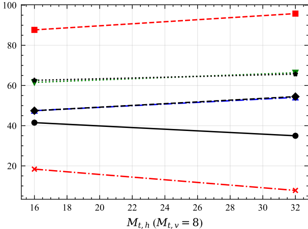
Sum-rate R [bits/s/Hz]
