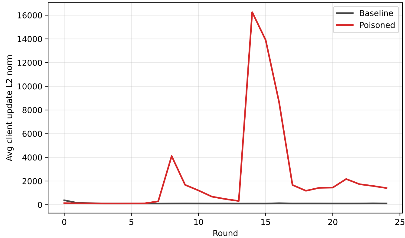
Average update norm (round-mean across selected clients)
