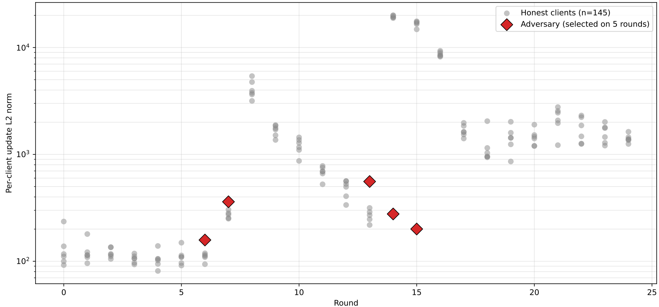
Per-client update norms: adversary vs. honest clients
